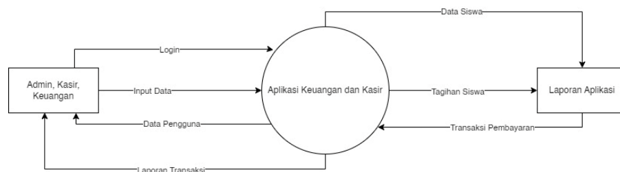
Gambar 3.5 DFD level 0
